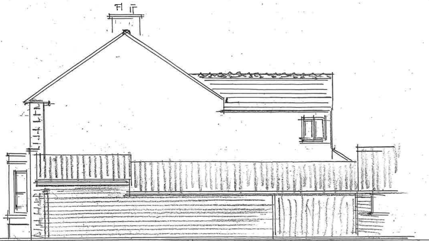
SITE ELEVATION (SOUTH)
